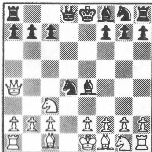
26 After 8 Qa4+
